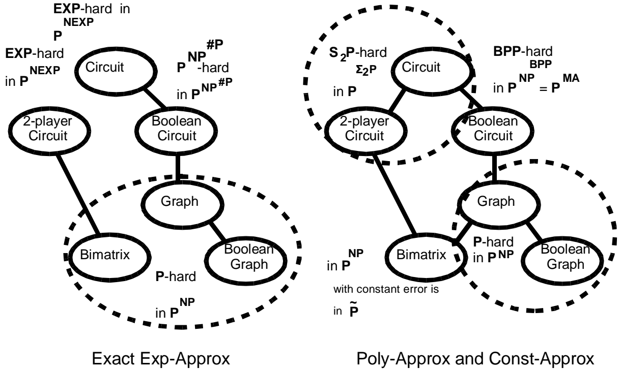
Figure 4: Summary of FINDNASH Results
